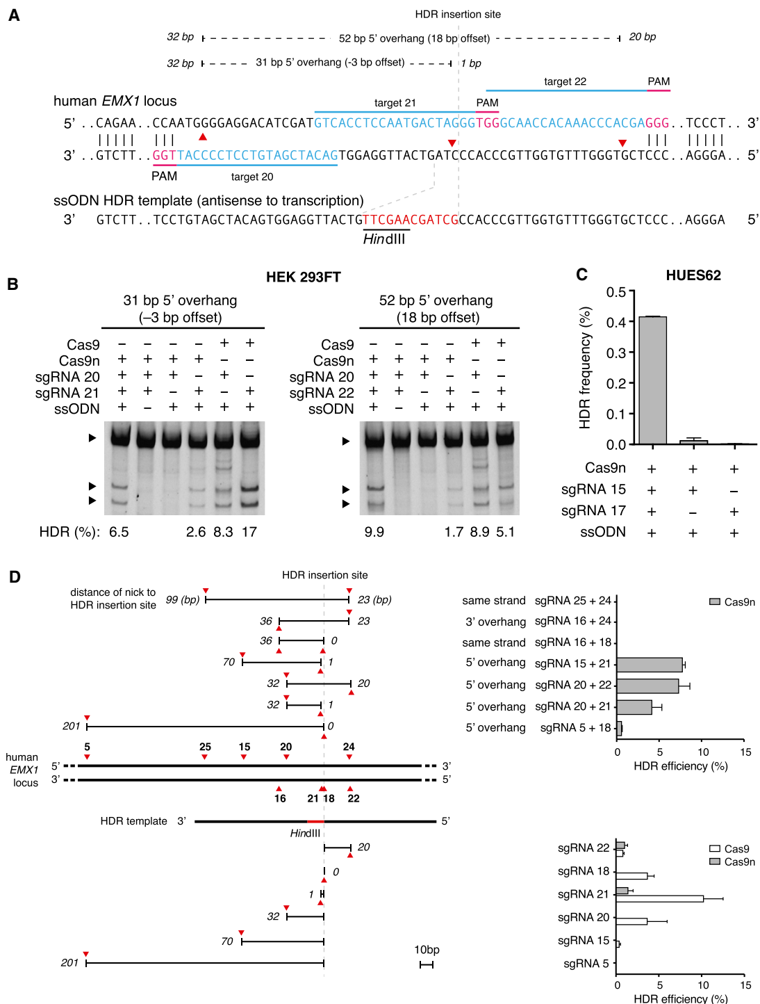
Figure 4. Double Nicking Allows Insertion into the Genome via HDR in Human Cells
